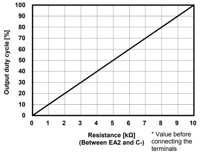
Resistance - Output Duty Cycle Characteristics
